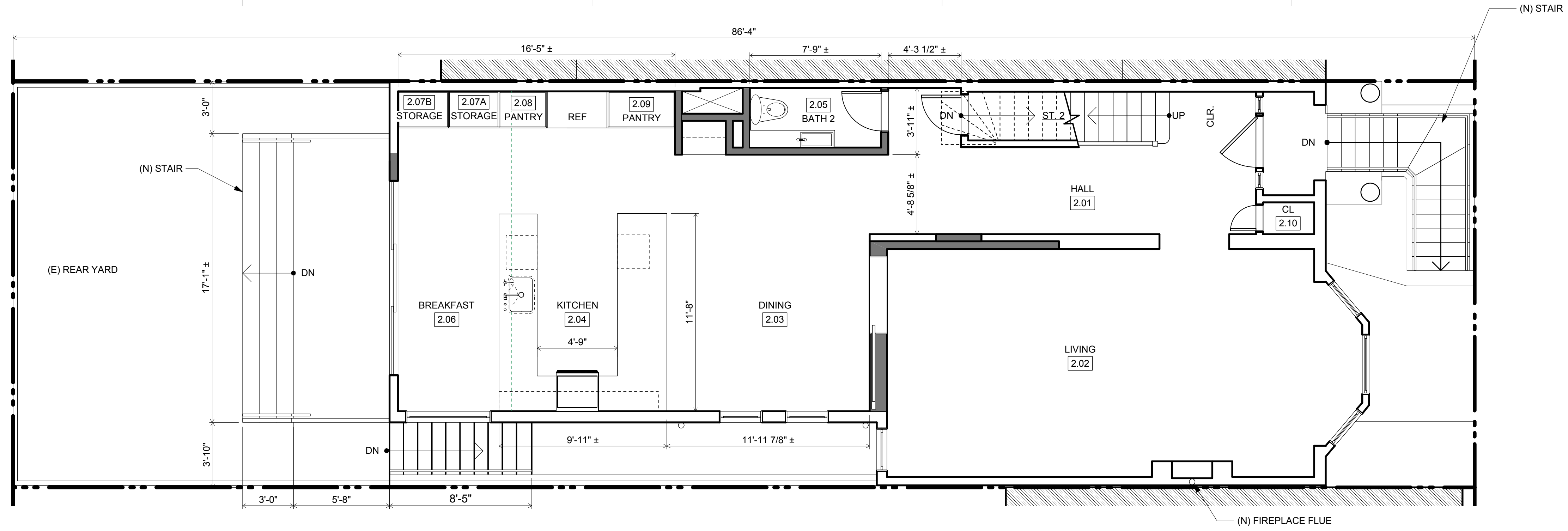
2 LEVEL 2 - PROPOSED Scale: 1/4" = 1'-0"
