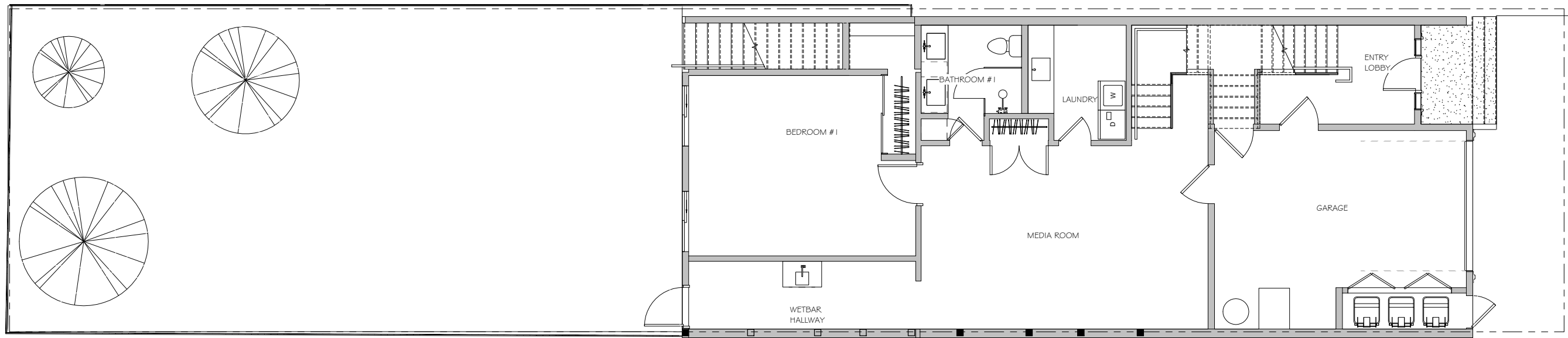
1 PROPOSED FL. PLAN - 1ST FLOOR 1/4" = 1'-0"
