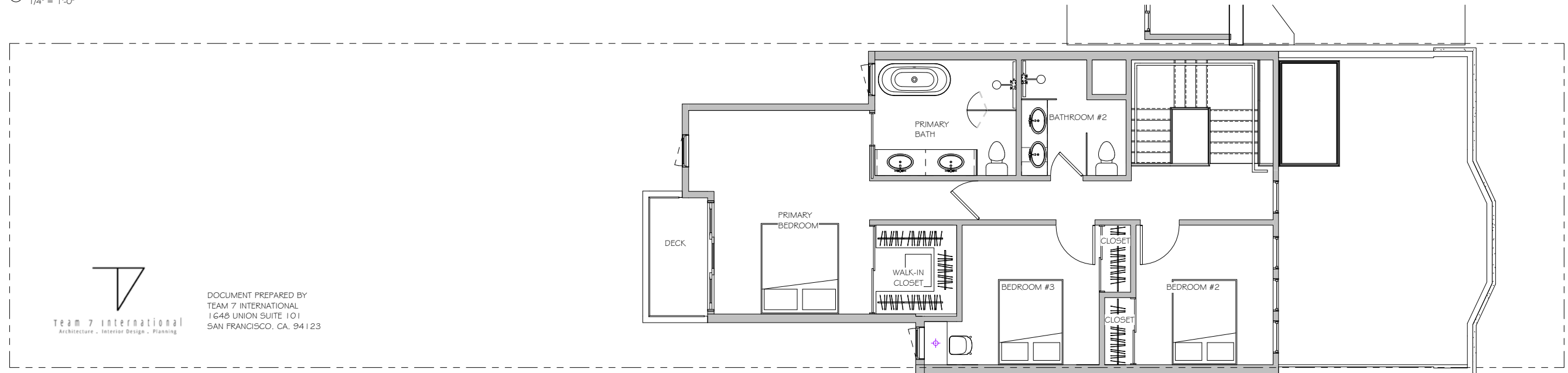
2 PROPOSED FL. PLAN - 2ND FLOOR 1/4" = 1'-0"
