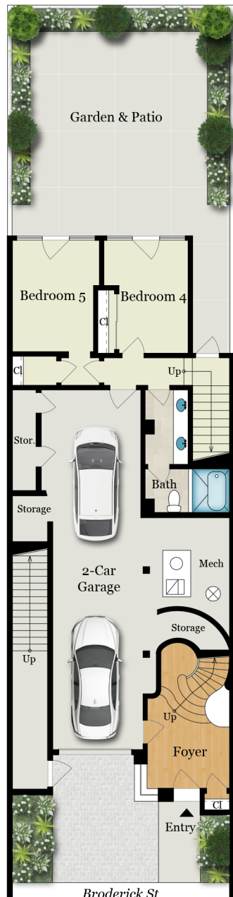
FIRST FLOOR
